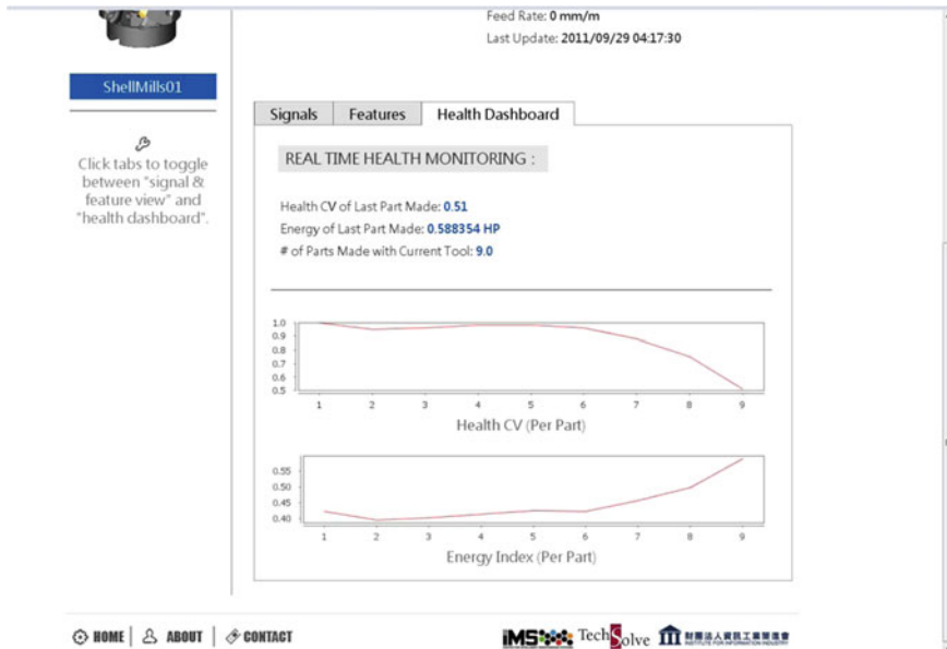
Fig. 60.9 A screenshot of the cloud-based prognostics for the tool insert (the horizontal axis indexes are the order of cuts)
