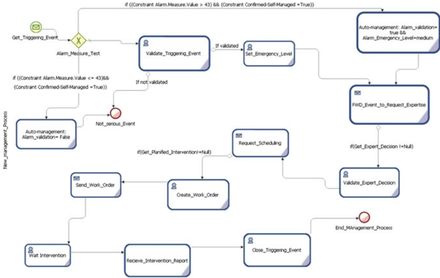
Fig. 44.7 New version of management process's workflow
