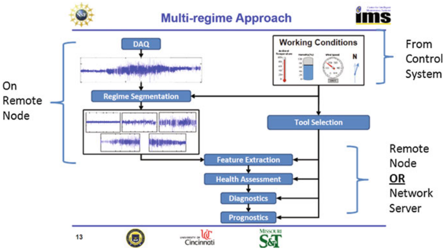
Fig. 19.4 IMS center multi-regime approach
