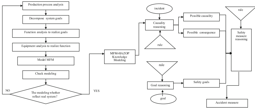
Fig. 51.1 How to build the MFM-HAZOP model
