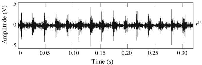
Fig. 27.4 r^{(1)} of the decomposition result using IRSGWT of the vibration signal for state 3
