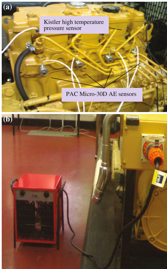
Fig. 24.1 Graphical illustration of the diesel engine test rig and sensors; the test rig (a) and the industry fan heater (b)
