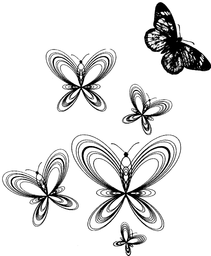
Figure 4.55 Butterfly curves.
