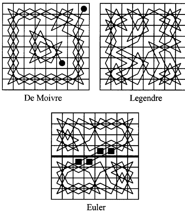
Figure 4.52 Knight's tours.
