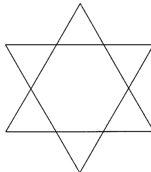
Figure 4.9 Draw the star without lifting your pencil and without repeating lines.
