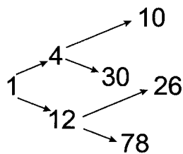
Figure 2.2 Grasshopper sequences.
