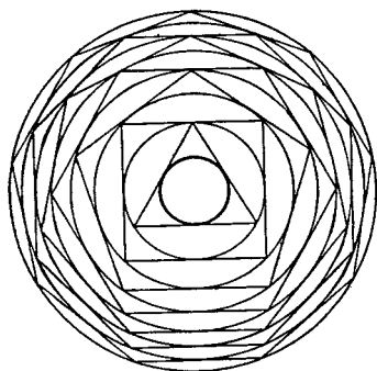
Figure 4.30 Infinitely exploding circles.
