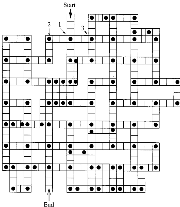
Figure 4.26 Aesculapian mazes.
