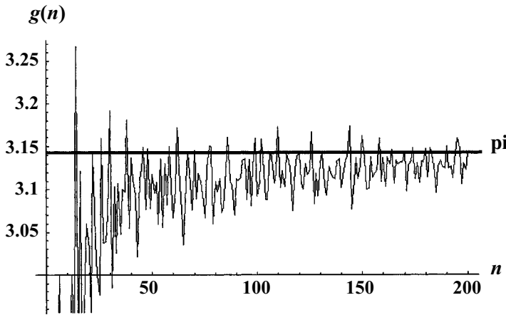
Figure 2.5 g(n) is a close approximation to \pi as n increases.
