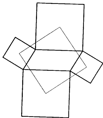
Figure 4.44 Thébault construction.
