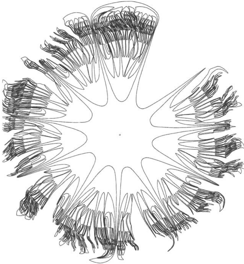
Figure 4.6 Symmetric II-Venn diagram, after removal of one of the curves, courtesy of Dr. Peter Hamburger of Indiana-Purdue University and Edit Hepp.
