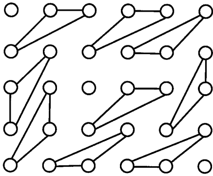
Figure A4.13 Mystery triangles.
