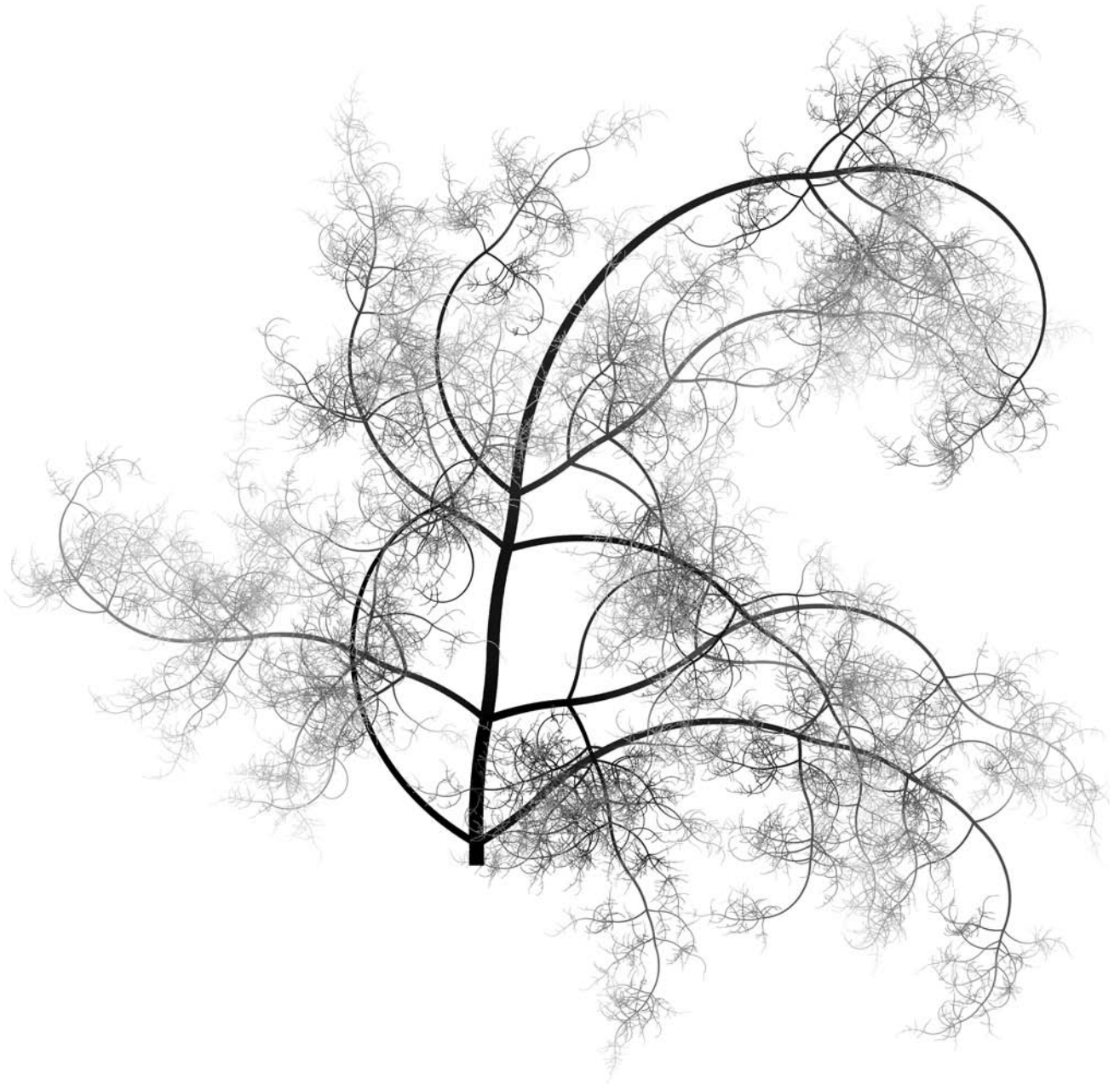
Figure 7.4 Tendrilous, botanical artwork produced by Chris Coyne using a simple set of mathematical rules. (See chriscoyne.com/cfdg/ for details.)
