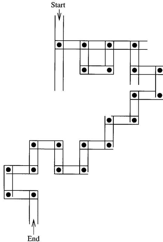
Figure A4.14 Aesculapian mazes.
