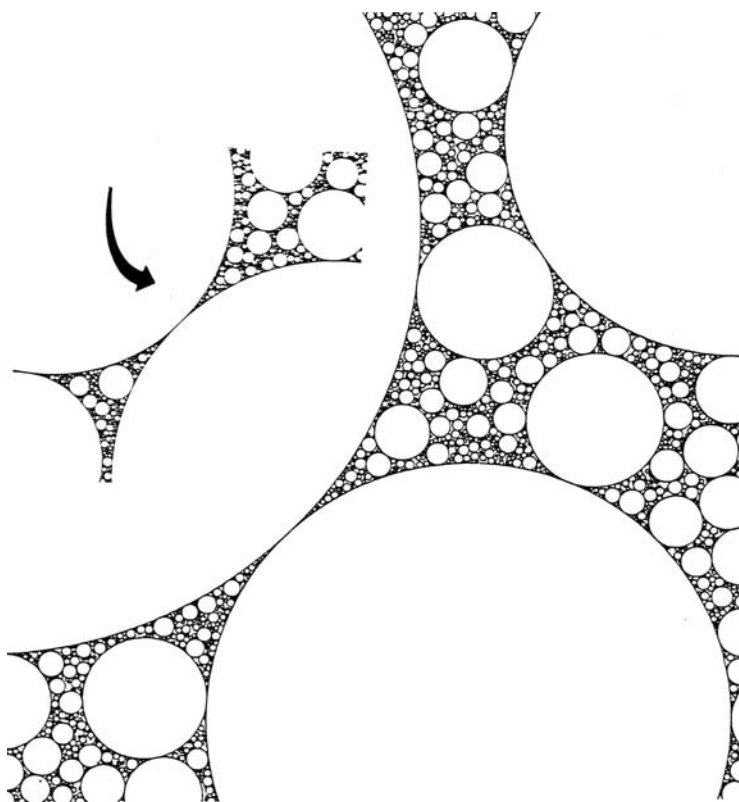
Figure 4.43 Osculatory circles.
