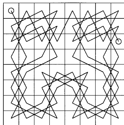
Figure 4.62 Knight’s path.
