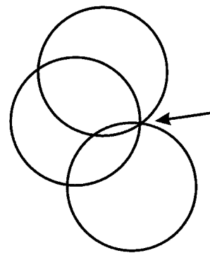
Figure 4.14 Circle crossing.
