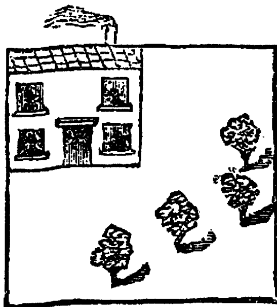
Figure 4.48 Dudeney’s house.
