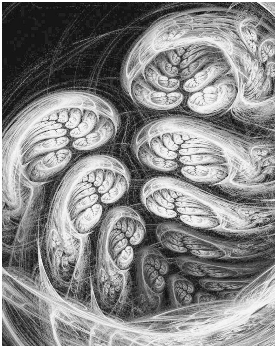
Figure 7.14 Fractal "Seed Pods," created by Cory and Catska Ench using an "iterated functions system" that consists of affine transformations involving rotations, scalings by a constant ratio, and translations. (See enchgallery.com for details.)
