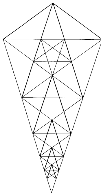
Figure 4.11 Mystery pattern.
