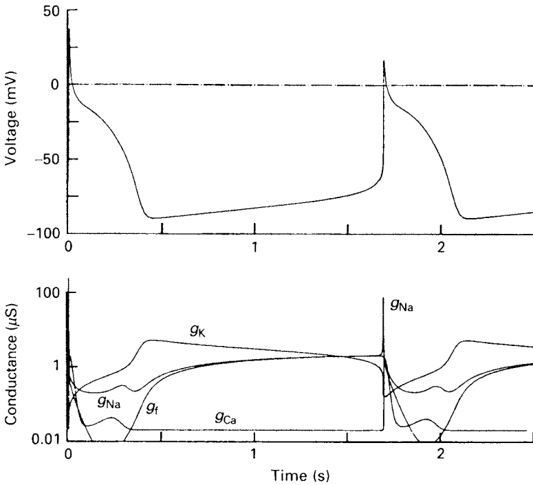
Fig. 11.3. Computer simulation of the cardiac action potential. The associated conductance changes are shown in the lower graphs: g_{\text{f}} is the inward current which becomes apparent during the pacemaker potential. The sodium conductance g_{\text{Na}} includes both the conductance due to fast sodium channels and the sodium component of g_{\text{f}} . From DiFrancesco and Noble (1985).
