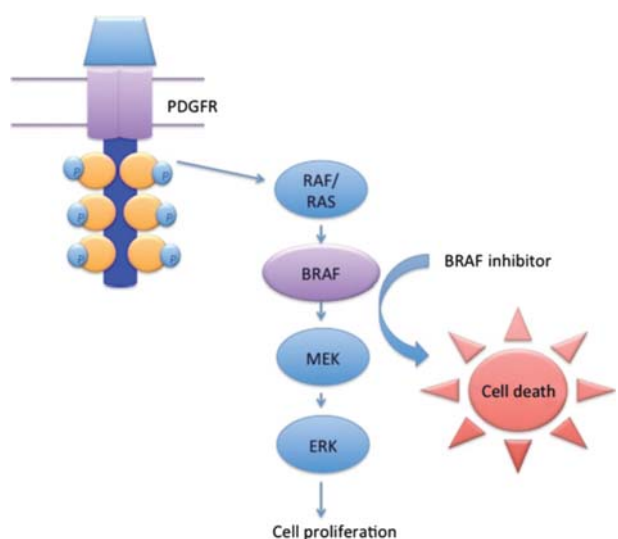
Figure 2. BRAF is a major protein intermediate in RAF/MEK.ERK signalling in normal cells but causes excessive proliferation in melanoma cells with BRAF mutations. The BRAF inhibitors cause cell death by apoptosis.
