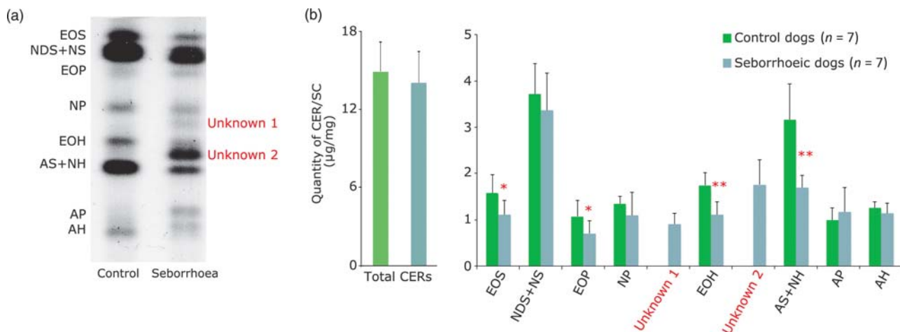
Figure 4. Skin surface ceramide (CER) profiles in shih tzu dogs with seborrhea and control dogs. (a) Representative data of HPTLC analysis of free extractable CER fractions in shih tzu dogs with seborrhea and control dogs. Two aberrant fractions (unknown 1 and unknown 2) are recognized exclusively in dogs with seborrhea. (b) Comparison of quantities of total CERs and CER fractions in control dogs and seborrheic dogs. Quantities of total CERs are not significantly different between the two groups. Quantities of CER[EOS], CER[EOP], CER[EOH] and a mixture of CER[AS] and CER[NH] were significantly lower in dogs with seborrhea than those in control dogs (* P < 0.05 , ** P < 0.01 , Student's unpaired t -test). Two unknown fractions are recognized exclusively in seborrheic dogs. Abbreviations: CER[EOS], combination of \omega -hydroxy fatty acids and sphingosines; CER[EOP], combination of \omega -hydroxy fatty acids and phytosphingosines; CER[EOH], combination of \omega -hydroxy fatty acids and 6-hydroxylsphingosines; CER[AS], combination of \alpha -hydroxy fatty acids and sphingosines; CER[NH], combination of nonhydroxy fatty acids and 6-hydroxyl sphingosines.
