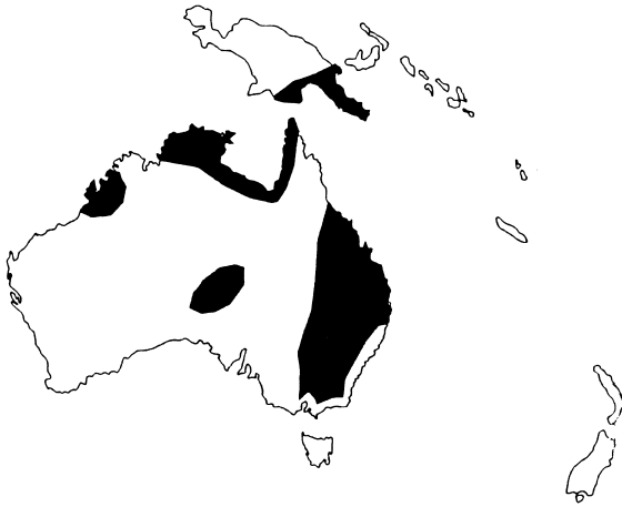
Figure 17.8 Geographic distribution of Murray Valley encephalitis virus
